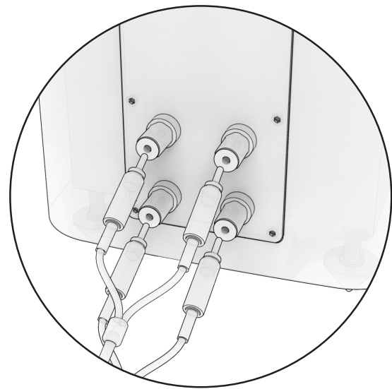
Bi-wiring or bi-amplification
